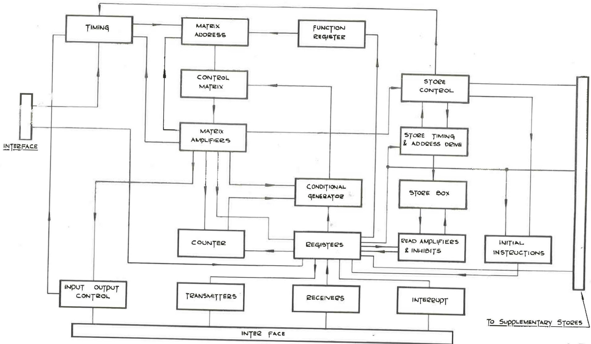
MCS 920B COMPUTER BLOCK DIAGRAM
